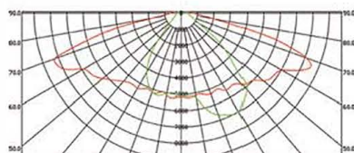
T II (80°*150°)
