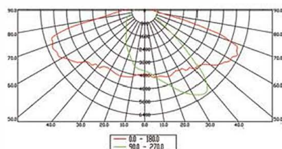
T III-2 (50° * 145°)
