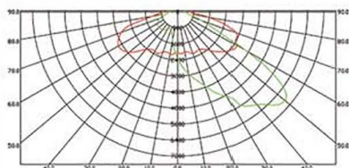
T III-1 (45°*155°)
